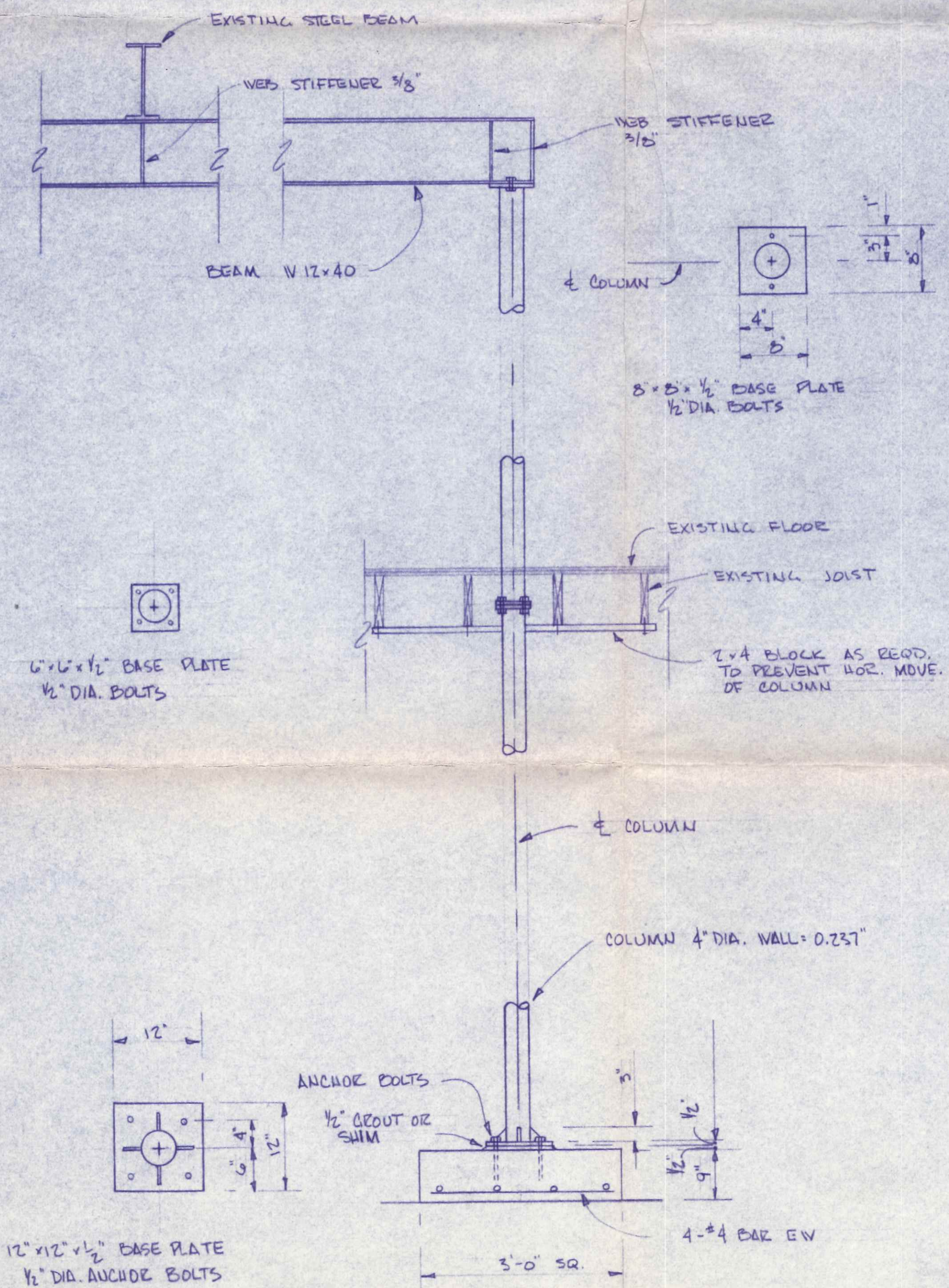
SECTION A-A 3/4" = 1'-0"
